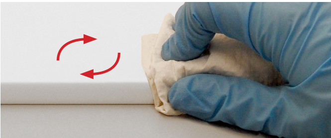
5. Polish the surface energetically with the specific product (B) until the surface gets its initial brightness
