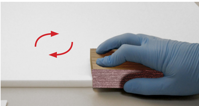
3. Sand the surface involved with a wooden block (B) and P500 sandpaper (A), following the direction shown.
